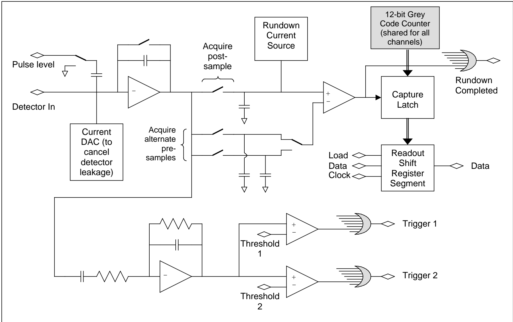
ACE "Matrix" Readout ASIC – Simplified Channel Block Diagram
